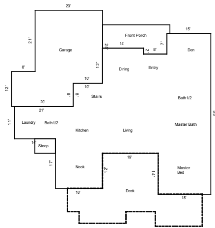
First Floor [2325 Sq Ft]
