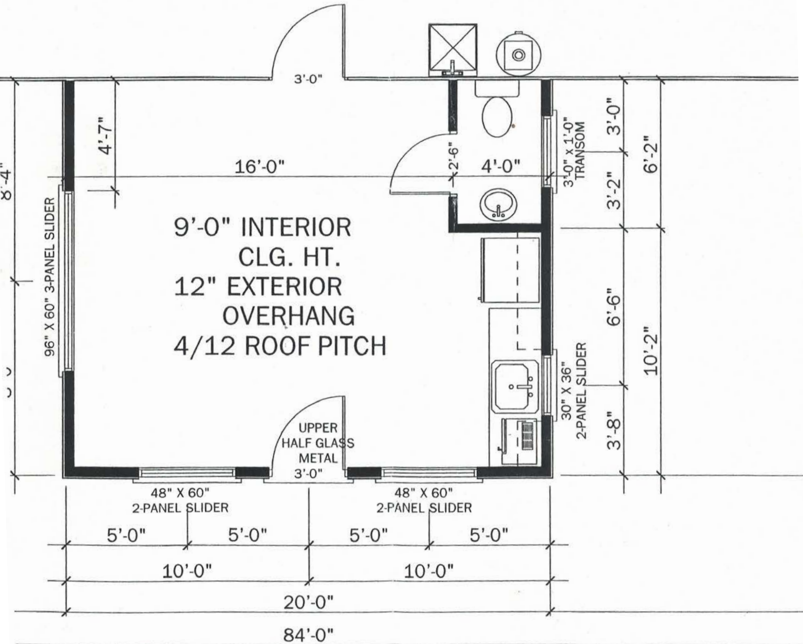
FLOOR PLAN — SCALE: \frac{1}{4}" = 1'-0"
