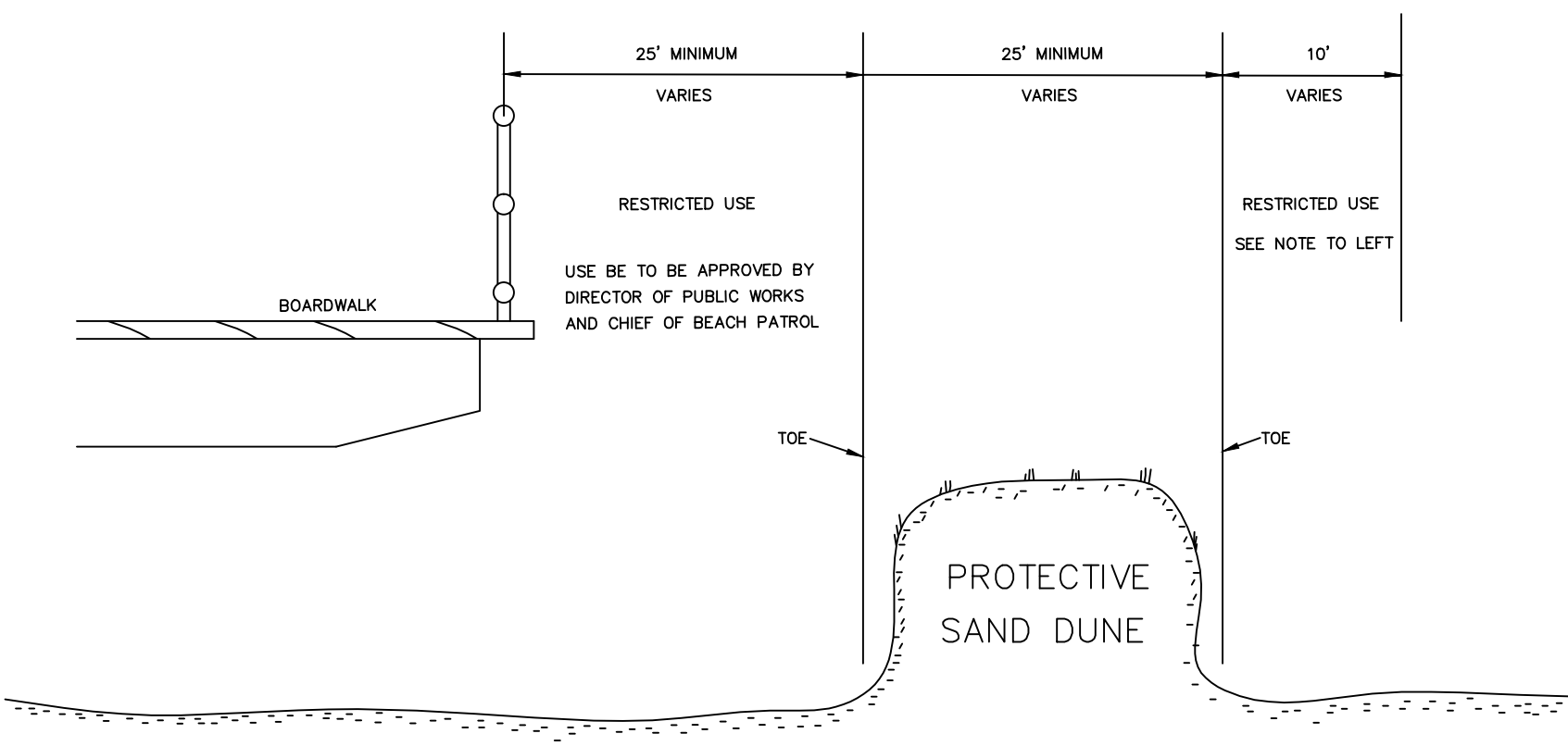
TYPICAL BEACH ELEVATION NO SCALE
