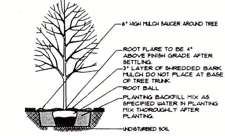
1 DECIDUOUS TREE PLANTING NOT TO SCALE
